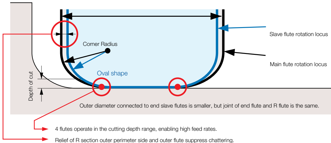
Turbo mill axial cross-section diagram
